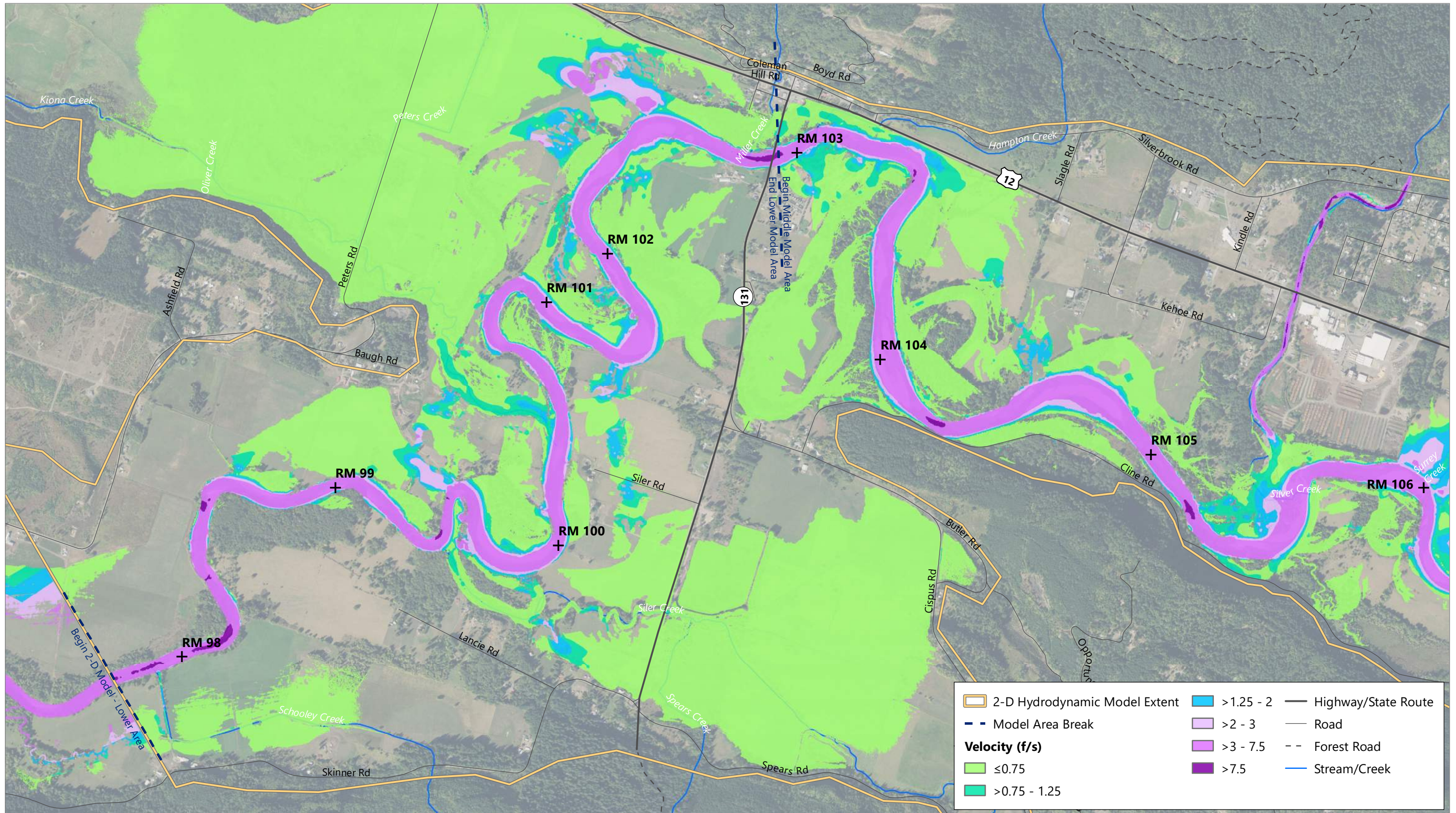
Figure 1 10-Year Flood Velocity Cowlitz River Restoration
